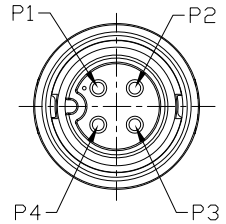
Pin Assignment
