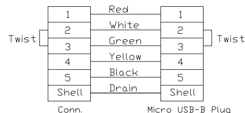
Wiring Diagram
