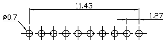
Recommended PCB Layout (PCB Board Tolerance ±0.05)
