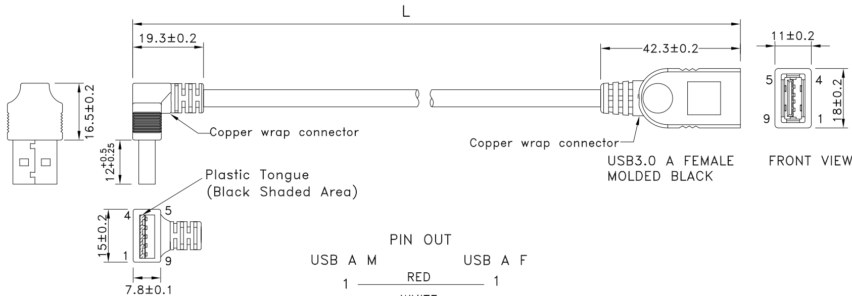
USB3.0 A MALE RIGHT ANGLE UP MOLDED BLACK
