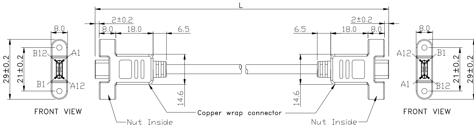
P1 USB TYPE C F MOLDED BLACK
