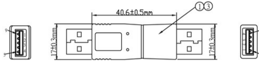
USB AM(NICKEL PLATED)
