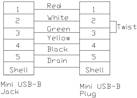
Wiring Diagram
